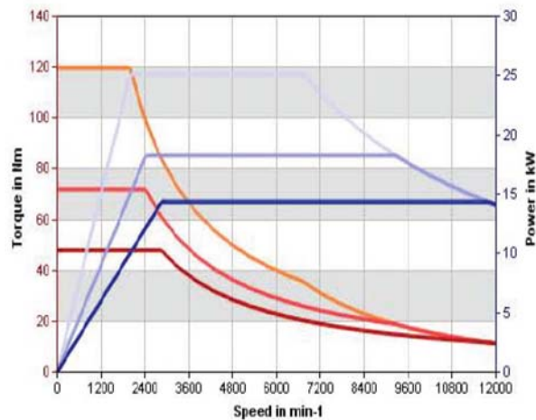
Characteristics of main drive
