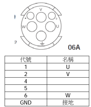
Power connector
